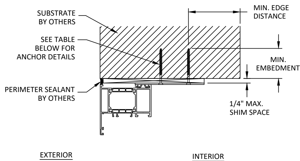
A 6 VERTICAL SECTION HEAD - STRAP
